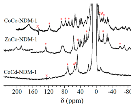
Figure 3. 200 MHz ^1\text{H} NMR spectra of Co(II)-substituted analogues of NDM-1 in 90% \text{H}_2\text{O} . Solvent-exchangeable protons are marked with asterisks. Transmitter imperfections are marked with an X.
